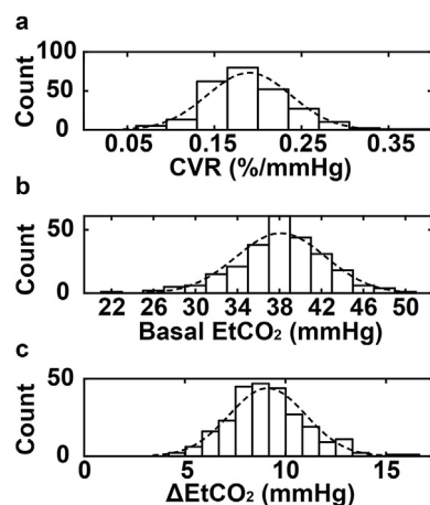
Fig. 2. The distributions of (a) whole-brain CVR, (b) basal \text{EtCO}_2 , and (c) \Delta\text{EtCO}_2 in the entire cohort ( N = 253 ). The Gaussian fittings of the histograms are also shown.
