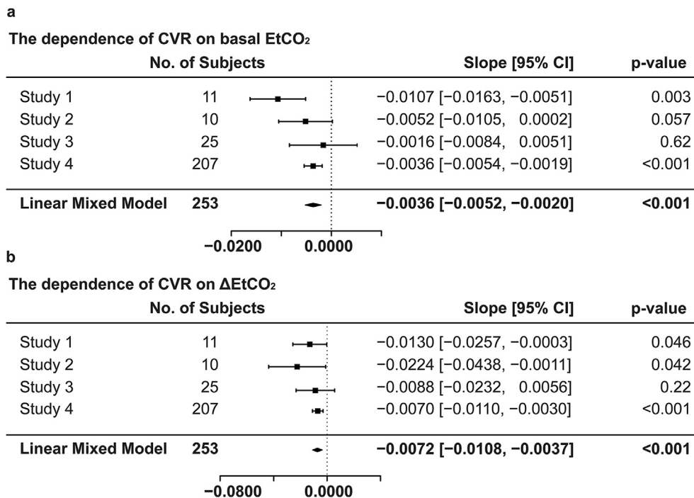
Fig. 3. Summary of the dependence of CVR on (a) basal EtCO 2 and (b) ΔEtCO 2 when considering each study separately and when combining all data.
